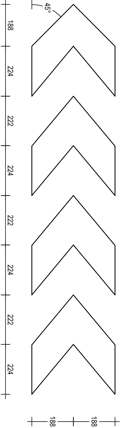
Symbol Detail
